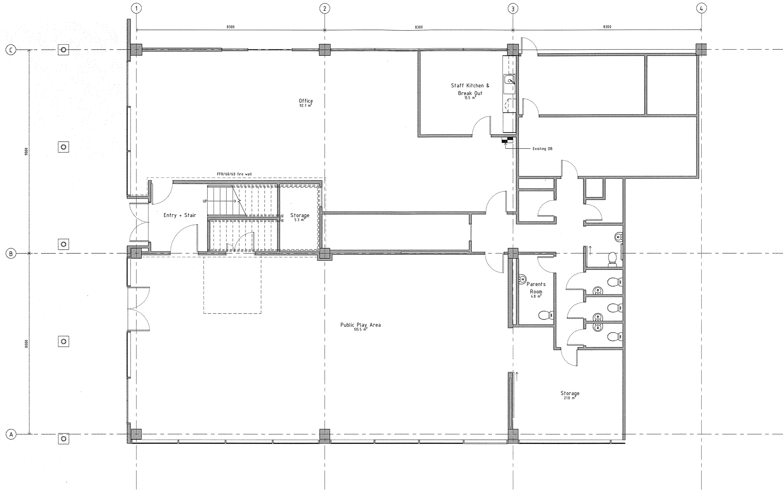
1 Existing Ground Floor Plan A4.20 1:50
